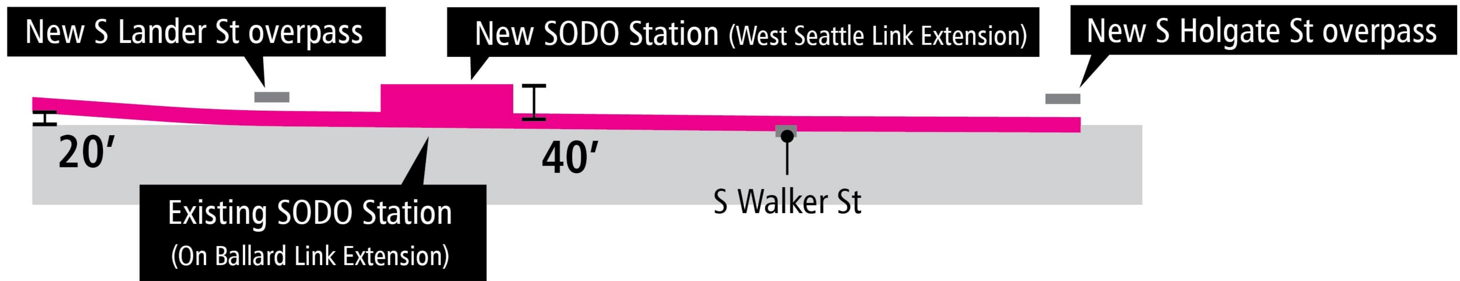
At-Grade Alternative (SODO-1a)
