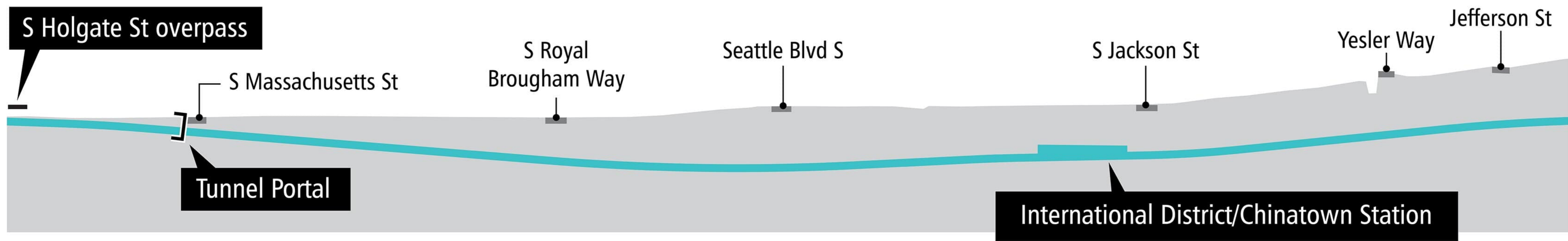
5th Avenue Shallow Alternative (CID-2a) Diagonal Station Configuration
